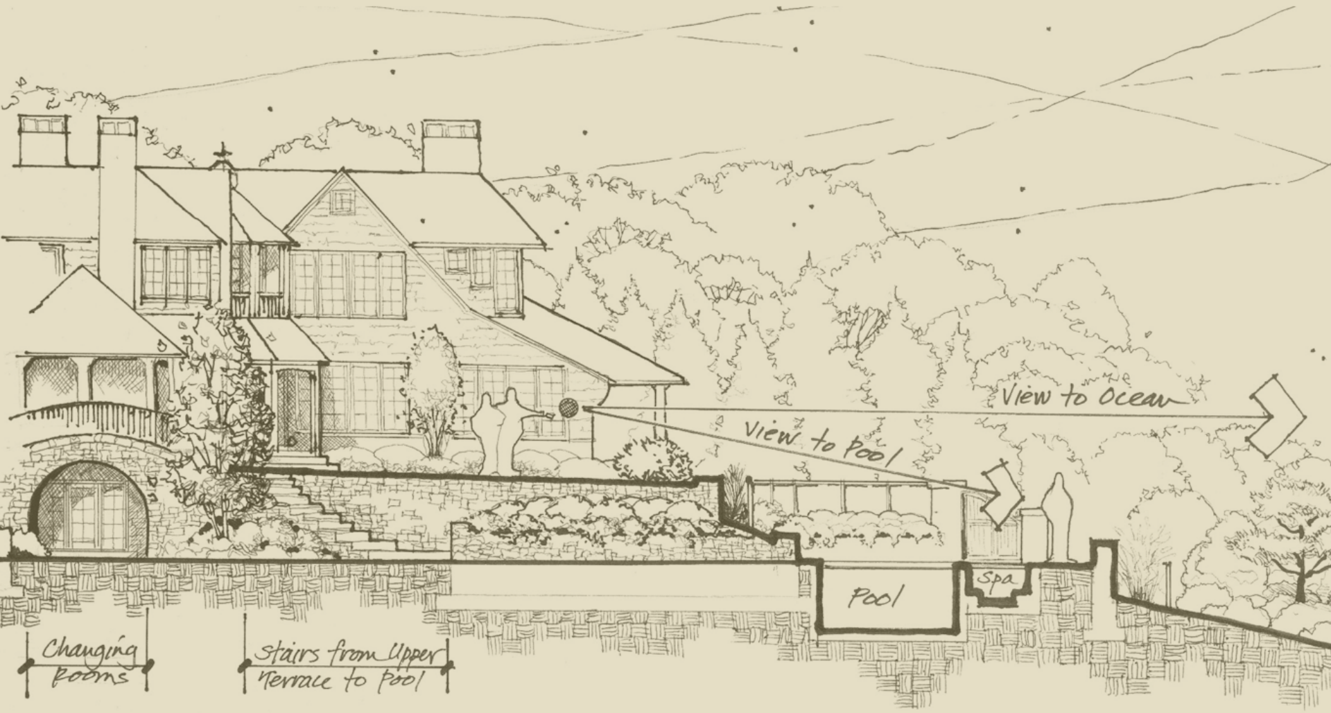
Section Elevation Through Terrace and Pool
